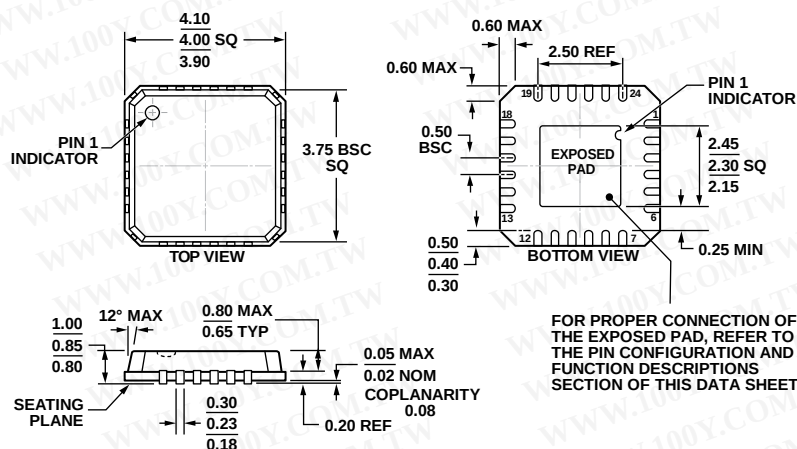
Figure 24. 24-Lead Lead Frame Chip Scale Package [LFCSP_VQ] 4 mm x 4mm Body, Very Thin Quad (CP-24-2) Dimensions shown in millimeters
